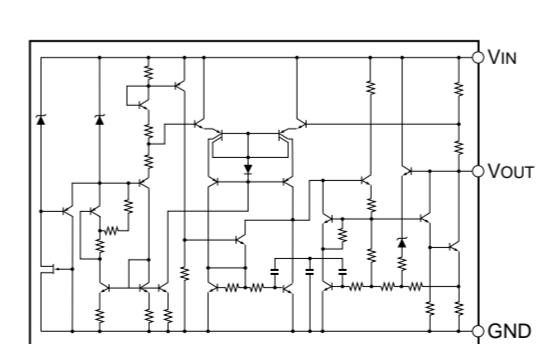
IC354: NJM78M05FA
