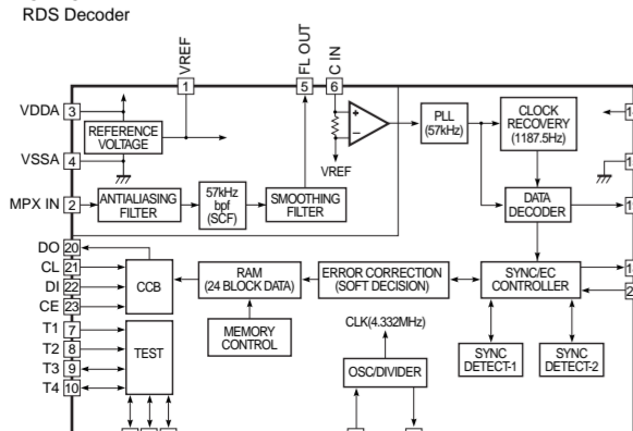
IC1: LC72722
